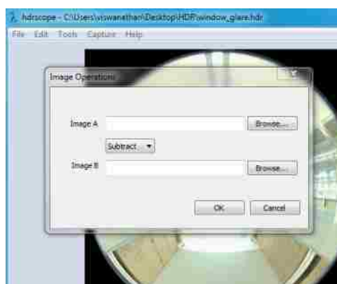
Figure 22 Image operations
